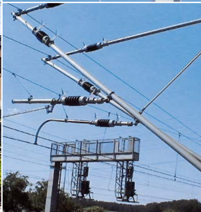
◀ RIBE® steady arms For all kinds of applications
